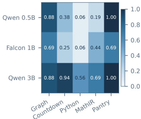
Absolute centered semantic mean (max)
