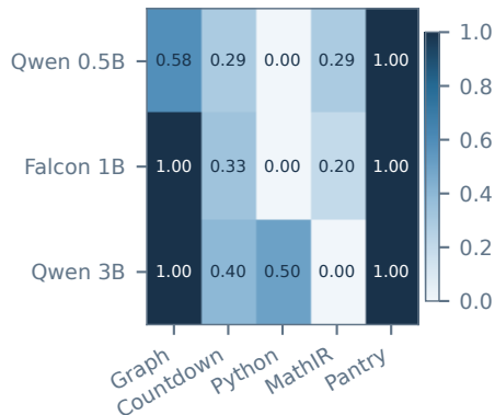
Applied replay score-gradient L2 (max)
