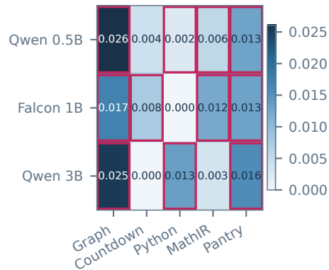
Verified-support semantic RMS (max)
