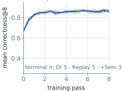
Qwen2.5-0.5B
