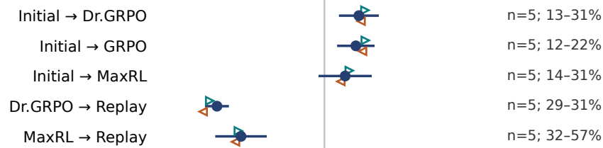
Qwen2.5-0.5B
