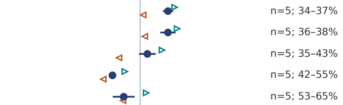
Qwen2.5-3B
