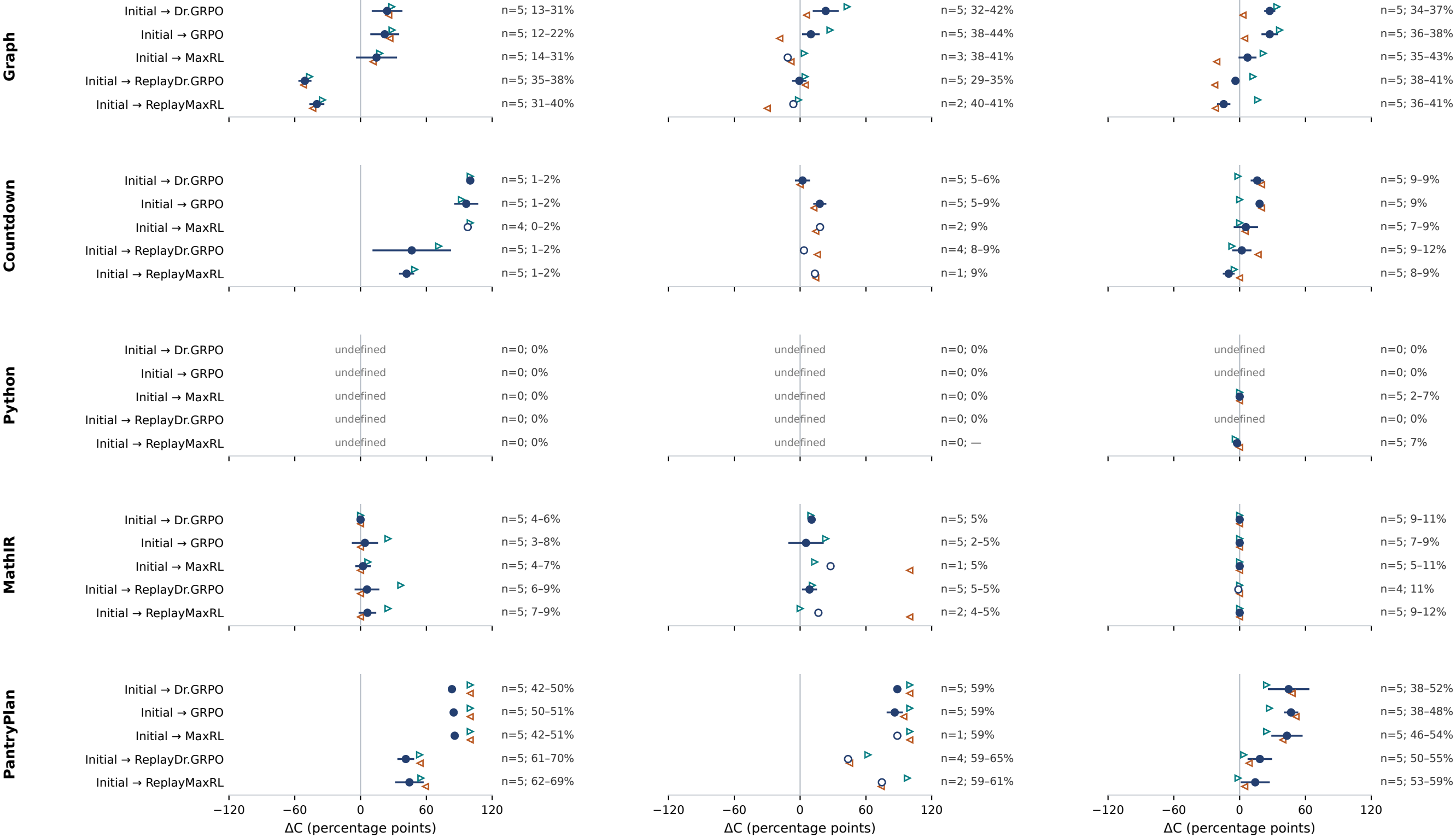
Qwen2.5-0.5B
