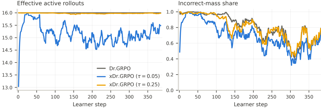
Figure 3: Candidate-level exploration diagnostics. Effective number of active rollouts \exp(H(a_x)) (left; uniform aggregation sits at the number of valid rollouts per group) and incorrect-mass share (right) over training. Lines are means over the three training seeds, bands are seed min–max, and both quantities are computed from the realized aggregation weights logged identically for every method in the quartet.
