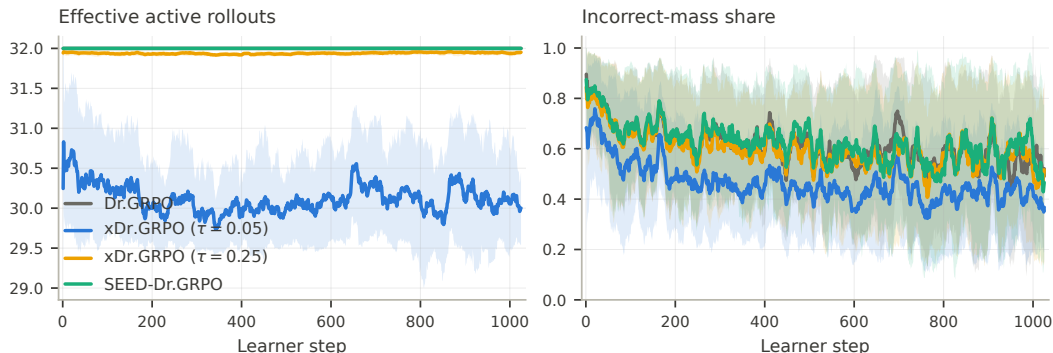
Figure 2: Candidate-level exploration diagnostics at 3B (graph coloring, G = 32 ; lines are means over three training seeds, bands seed min–max, computed from the realized aggregation weights logged identically for every arm). Effective number of active rollouts \exp(H(a_x)) (left) and incorrect-mass share (right) over training: tempered aggregation at \tau = 0.05 concentrates only mildly while consistently attenuating the weight on incorrect candidates, reproducing the 0.5B mechanism of Figure 3 at scale.
