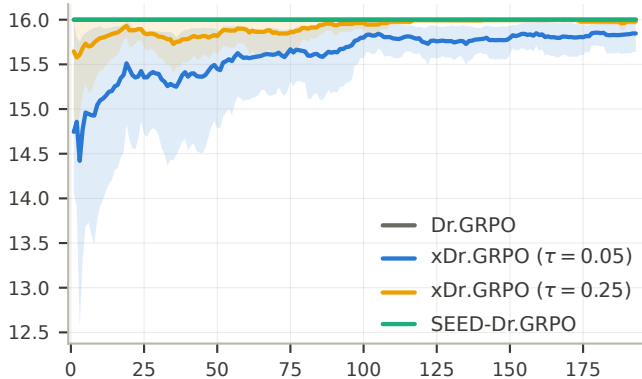
Effective active rollouts — 3B (G=32)
