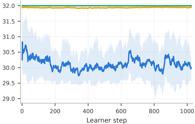
Effective active rollouts — 3B (G=32)
