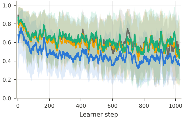
Incorrect-mass share — 3B (G=32)
