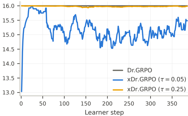
Effective active rollouts
