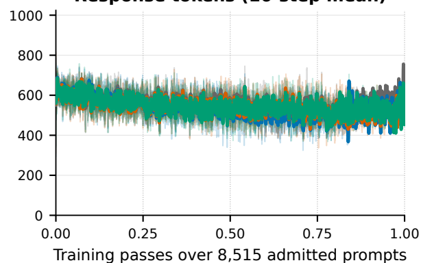
Response tokens (16-step mean)
