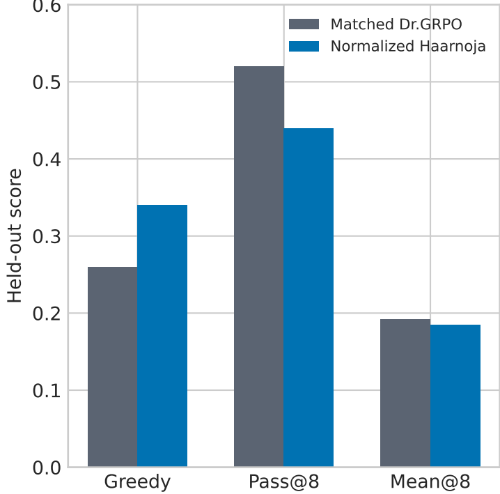
C. First matched toy after 3 epochs
