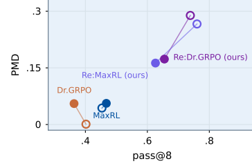
Figure 9: Replay across difficulty levels at Qwen2.5-0.5B. Open/filled markers denote Level 1/2; both levels and all four methods share five paired seeds. pass@8 averages all five domains; PMD averages the two — Graph and MathIR, with Graph dominating — where every method clears the support bar at both levels, so no arm rests on an easier subset than its control (App. F.3).
