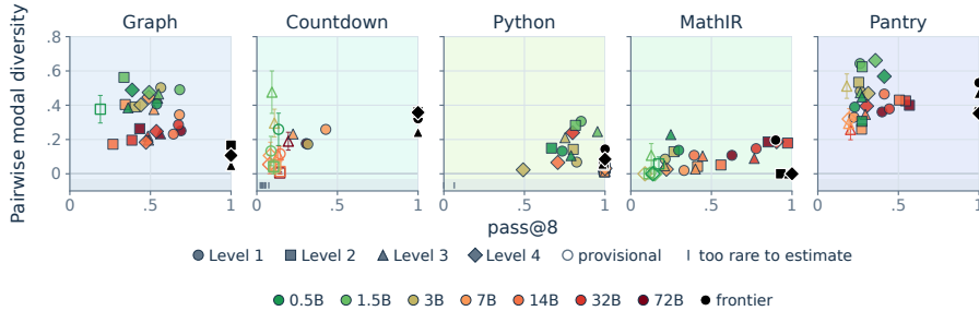
Figure 3: Breadth narrows as problems get harder and as models get larger. Frozen Qwen2.5-Instruct scales: colour is parameter count, marker shape is the level. PMD falls with level, falls again with scale, and falls for the frontier models of Section 2.3 (black, off the size ramp) from .270 to .188 — while they answer .991 of prompts correctly at every level, so their narrowing is not a side effect of failing more. Hollow markers carry PMD below the support bar, with its standard error; ticks mark measurements too rarely solved to place.
