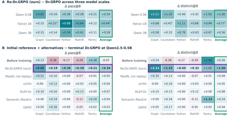
Figure 7: Canonical replay improves correctness and verified breadth. (A) Re:Dr.GRPO minus Dr.GRPO at all three scales. (B) Qwen2.5-0.5B alternatives minus Dr.GRPO. Columns measure probability points and expected verified-mode counts, respectively. The green Average weights domains equally within seed. A dagger marks four paired seeds in Falcon Countdown and its Average; the rest use five. Intervals are nominal 95% intervals for five-seed comparisons. Purple denotes Re:Dr.GRPO; bold entries mark column maxima in Panel B.
