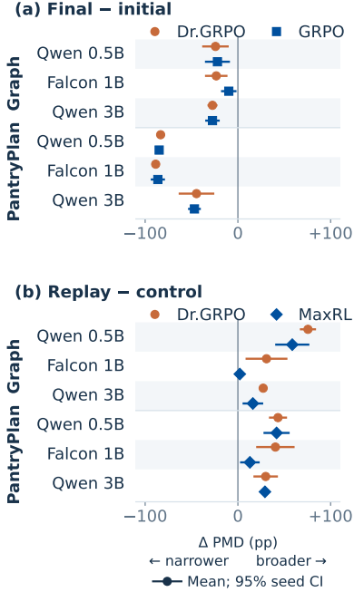
Figure 6: Training concentrates verified outputs; replay reverses it. Narrower is left, broader is right. (a) Change in PMD over training under Dr.GRPO and GRPO: all twelve move left. (b) Replay minus its matched control: all twelve move right. Graph and PantryPlan have enough initial breadth to define the measure. Dots and 95% intervals are five seed contrasts over jointly eligible prompts; panels have separate eligibility, and counts and magnitudes are in App. H.1.
