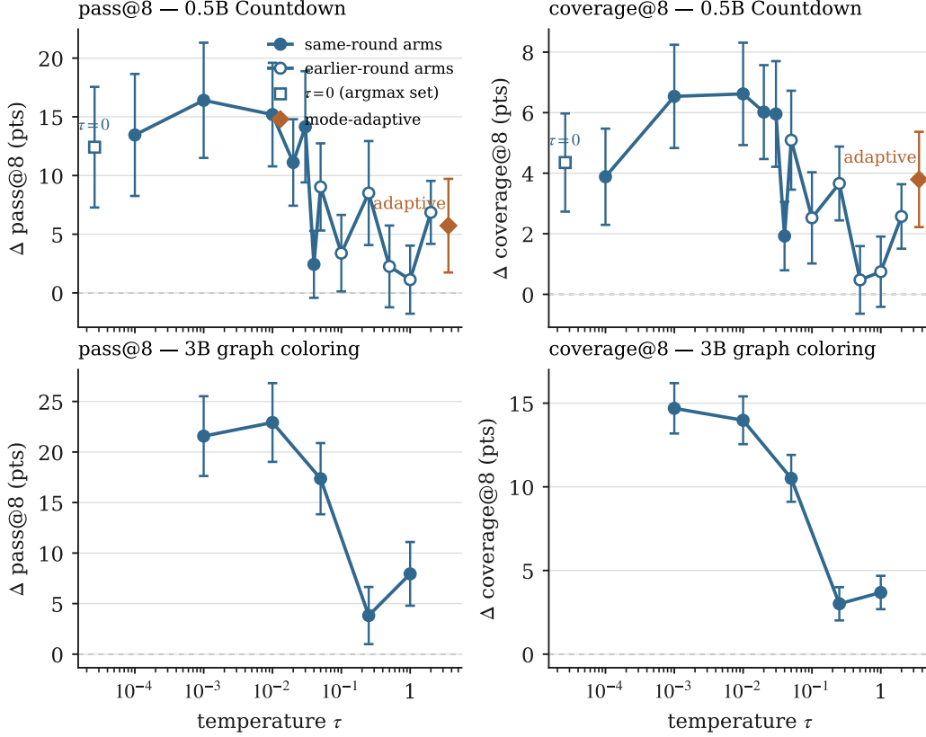
Figure 1: Dose-response of candidate-level tempering at both scales (multi-answer splits): treatment effect vs. Dr.GRPO with 95% prompt-clustered CIs, for pass@8 (left) and coverage@8 (right). Top row: 0.5B Countdown — filled markers: same-round arms; open markers: earlier-round arms; each round is estimated against its own matched baseline; the open square is exact argmax-set aggregation ( \tau = 0 ) and the diamond the mode-adaptive arm (no fixed abscissa). Bottom row: the 3B graph-coloring sweep. Both scales show the same shape — a rise to a plateau below \tau \approx 0.01 — with larger amplitudes at 3B. At 0.5B the plateau extends through exact \tau = 0 with no accuracy cost; at 3B the extreme end trades mean@8 for coverage (Section 5.3), so the accuracy-neutral optimum sits at \tau \approx 0.01 – 0.05 . Dashed lines mark zero.
