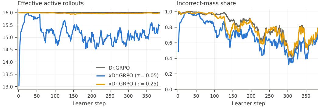
Figure 1: Candidate-level exploration diagnostics. Effective number of active rollouts \exp(H(a_x)) (left; uniform aggregation sits at the number of valid rollouts per group) and incorrect-mass share (right) over training. Lines are means over the three training seeds, bands are seed min–max, and both quantities are computed from the realized aggregation weights logged identically for every method in the quartet.
