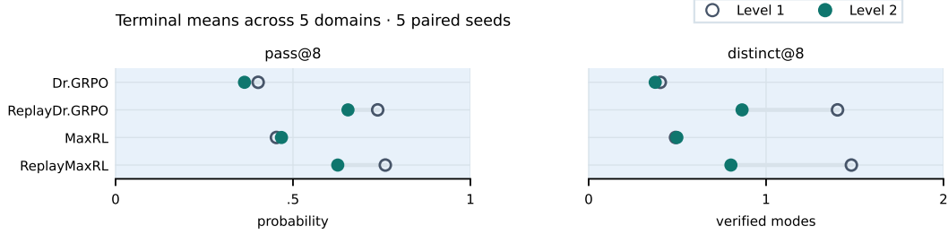
Figure 7: Replay across difficulty levels: Qwen2.5-0.5B-Instruct. Open/filled: Level 1/2. Means equally weight all five complete domains within five paired seeds shared across levels and methods (Appendix G.3). Archived models.
