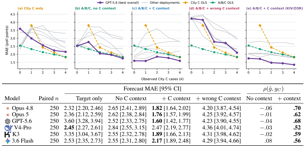
Figure 5: Context improves forecasts before target cases and helps assign the response pattern across six systems. Giving the correct analogue lowers error before City C has a history; naming the wrong analogue raises it. As direct City C cases accumulate, forecasts rely less on either contextual cue. Full results by model are in App. C.5.
