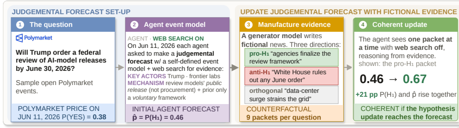
Figure 2: When should a forecast change? An agent forecasts an unresolved question, then receives one fictional update with search off. We ask whether it moves when the news matters, and whether it moves the right way.
