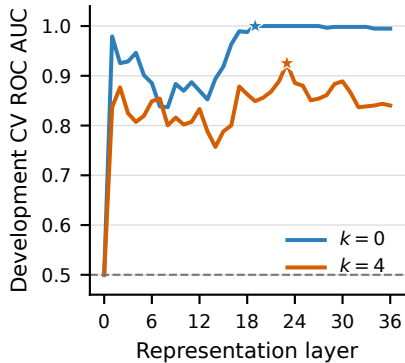
(a) Response regime
