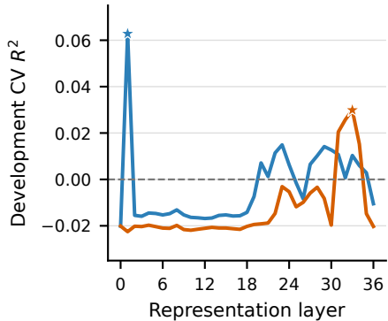
(c) Within-regime residual
