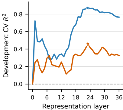
(b) Full latent slope
