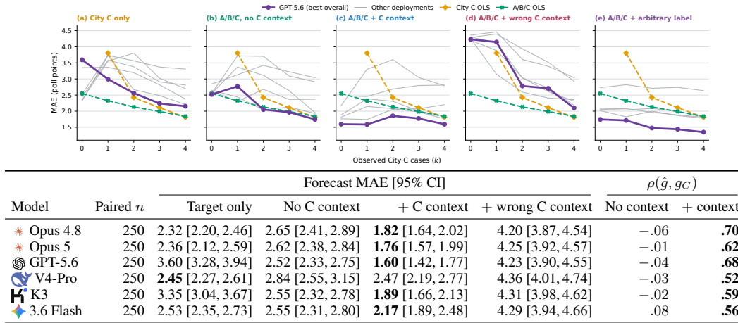
Figure 5: Context improves forecasts before target cases and helps assign the response pattern across six systems. Giving the correct analogue lowers error before City C has a history; naming the wrong analogue raises it. As direct City C cases accumulate, forecasts rely less on either contextual cue. Full results by model are in App. C.5.
