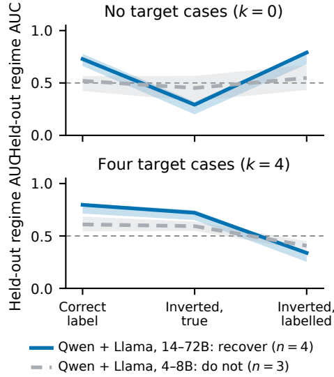
Figure 6: Larger models infer an episode-local convention, then yield to direct evidence. On 88 new episodes, four larger Qwen and Llama checkpoints (14–72B) encode the changing KIV/ZOR mapping; three smaller checkpoints (4–8B) do not reliably encode it. The decoded state follows context before City C has a history and follows the target relationship as local cases accumulate.
