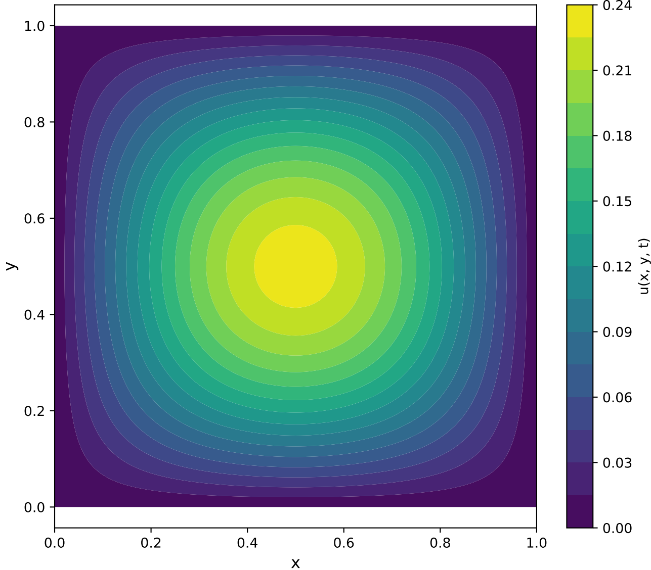
Numerical Solution at t=0.301
