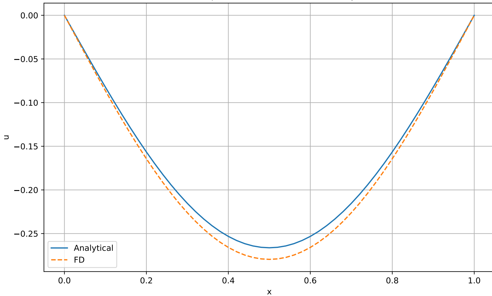
2D Wave Equation at final time (slice at y=0.5 )
