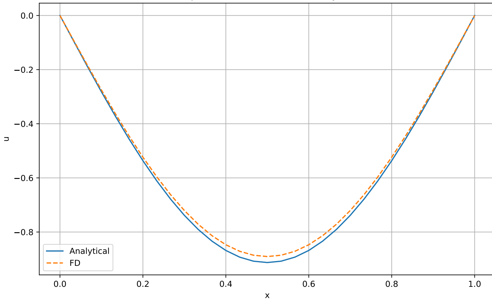
3D Wave Equation at final time (slice at y=0.5 , z=0.5 )
