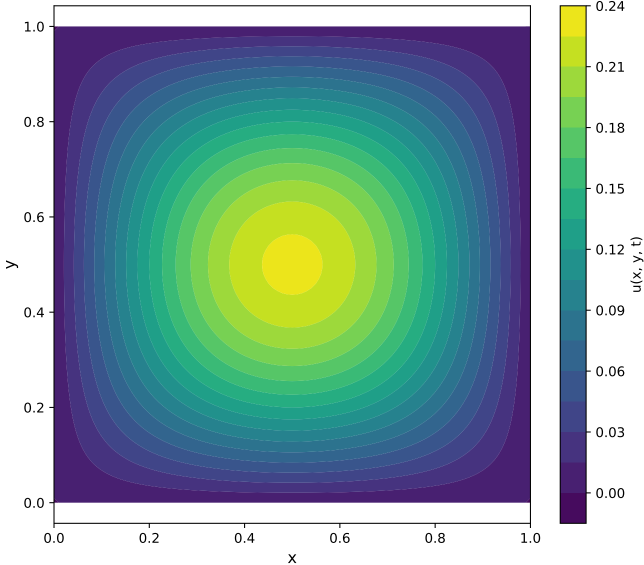
Exact Solution at t=0.301
