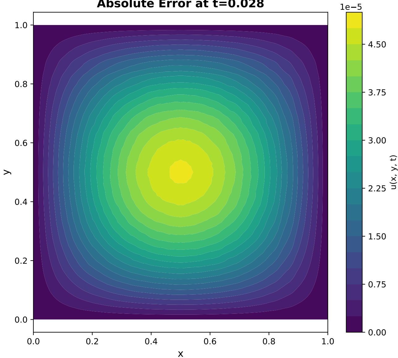
Absolute Error at t=0.028
