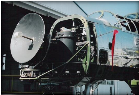
Early Dish Antenna (WWII)
