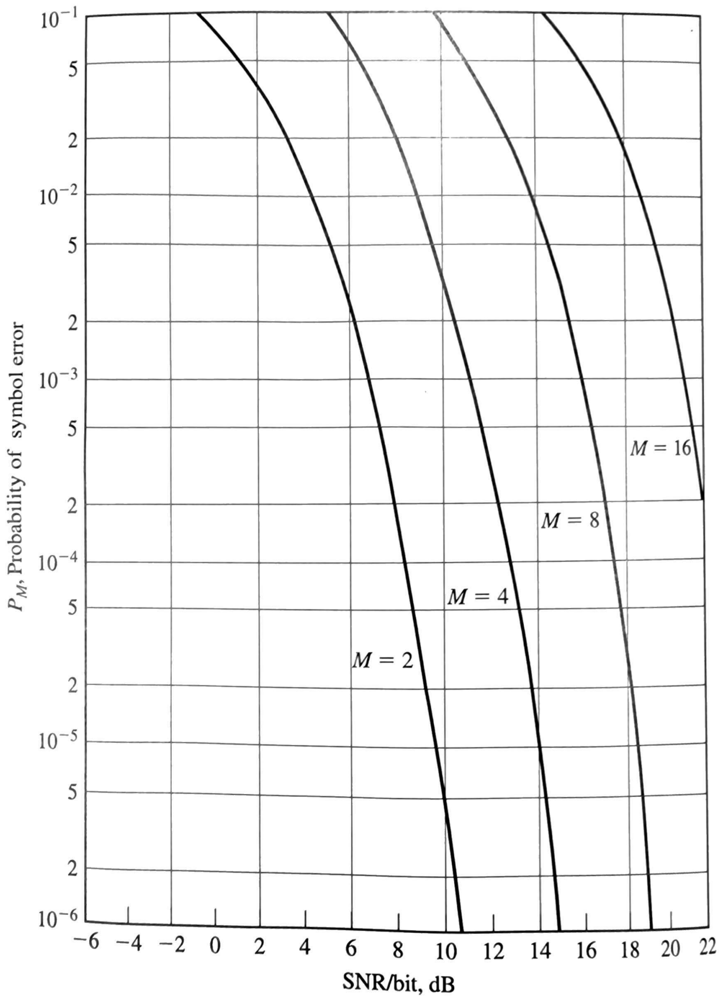
Figure 7.55 Probability of a symbol error for PAM.
