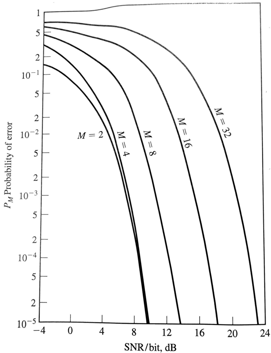
Figure 7.57 Probab error for PSK signals
