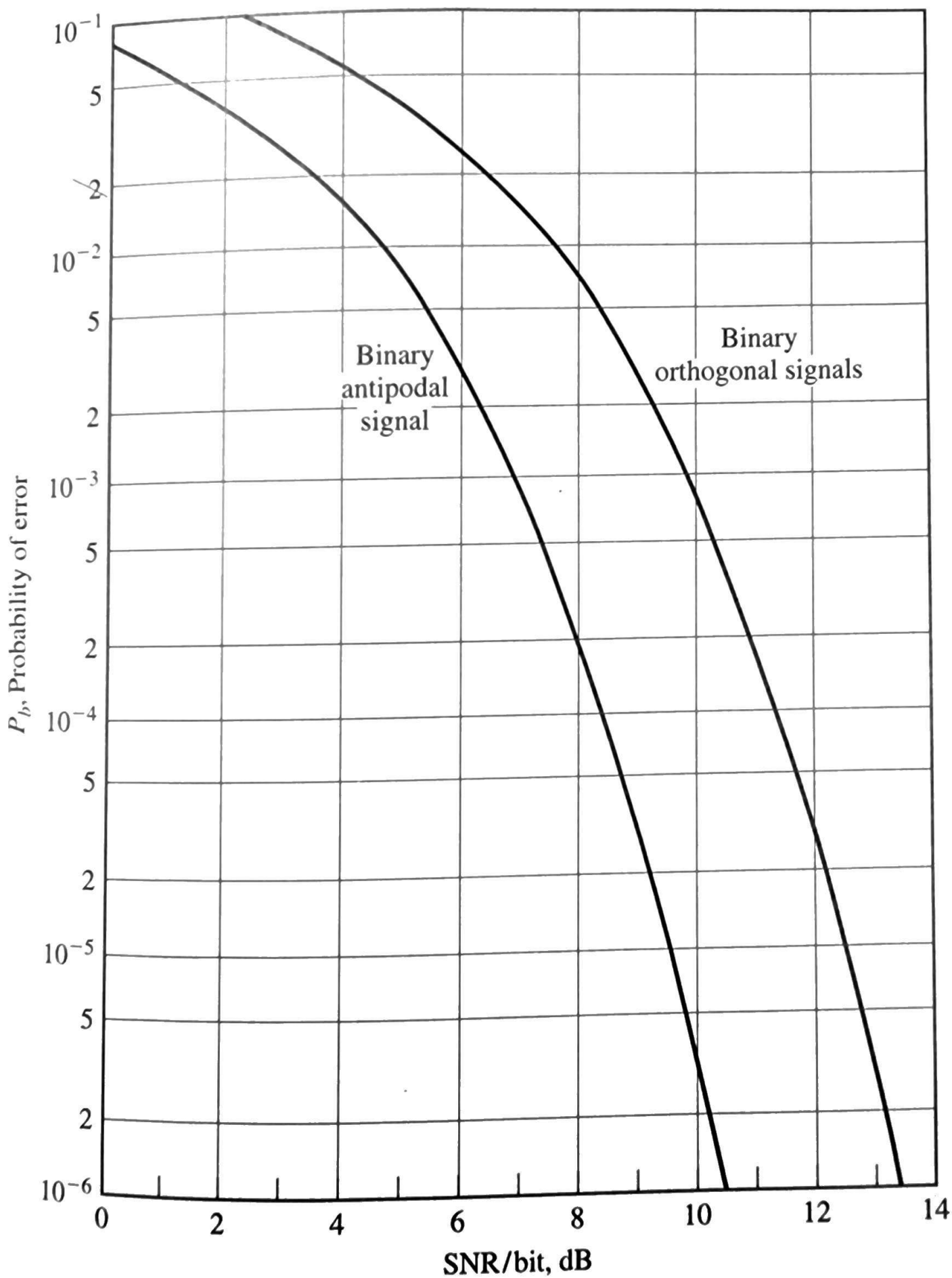
Figure 7.53 Probability of error for binary signals.
