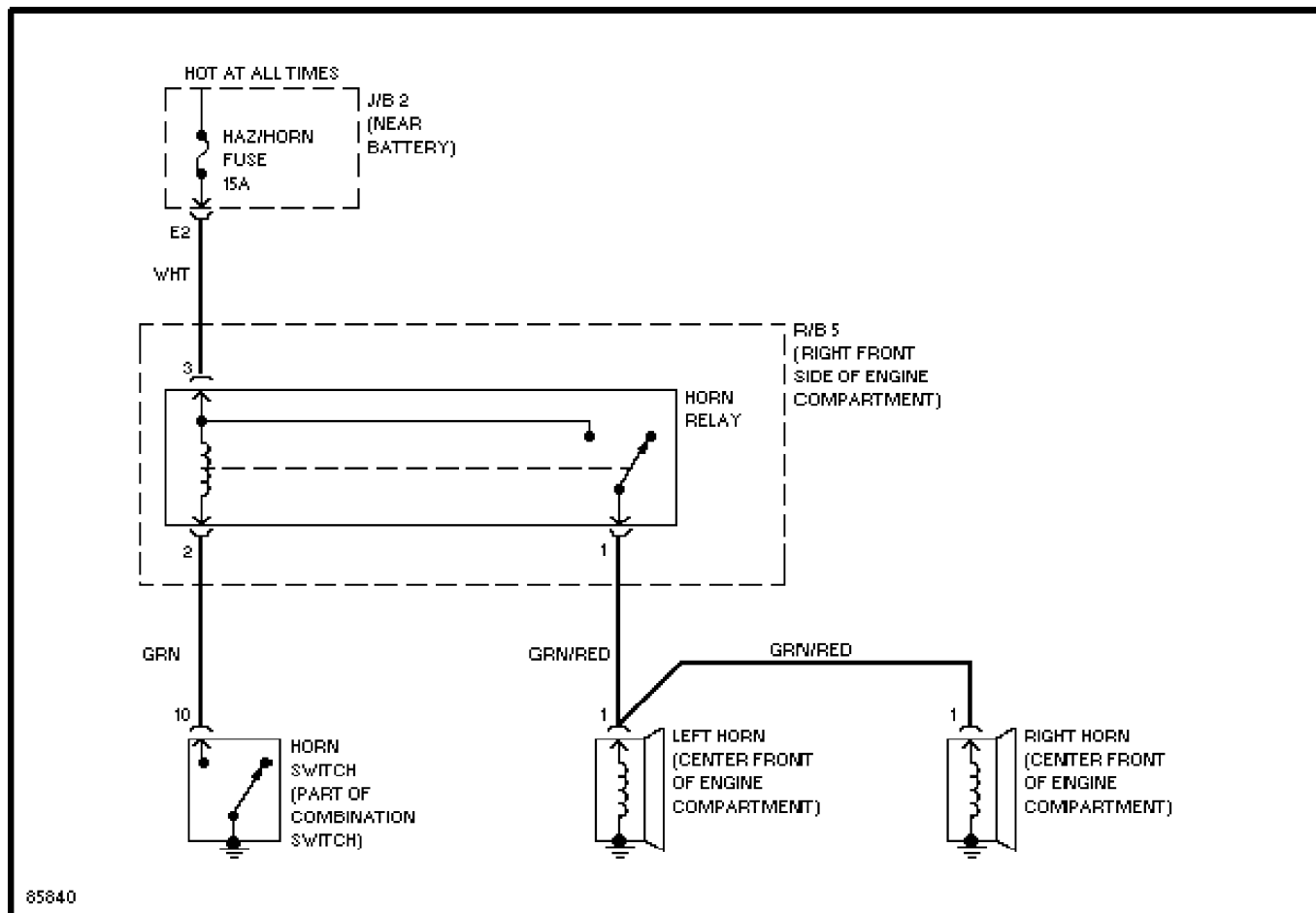
Horn Circuit
