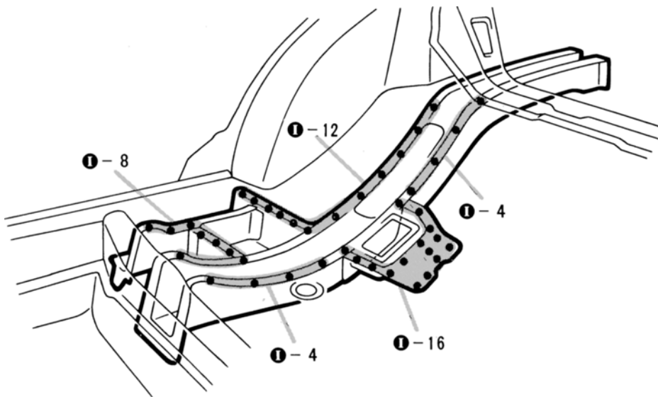
Rear Suspension Member Body Mounting Bracket.
