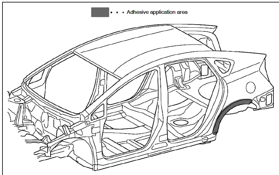
2012 Toyota Prius Adhesive Use on Rear Quarter Panel
