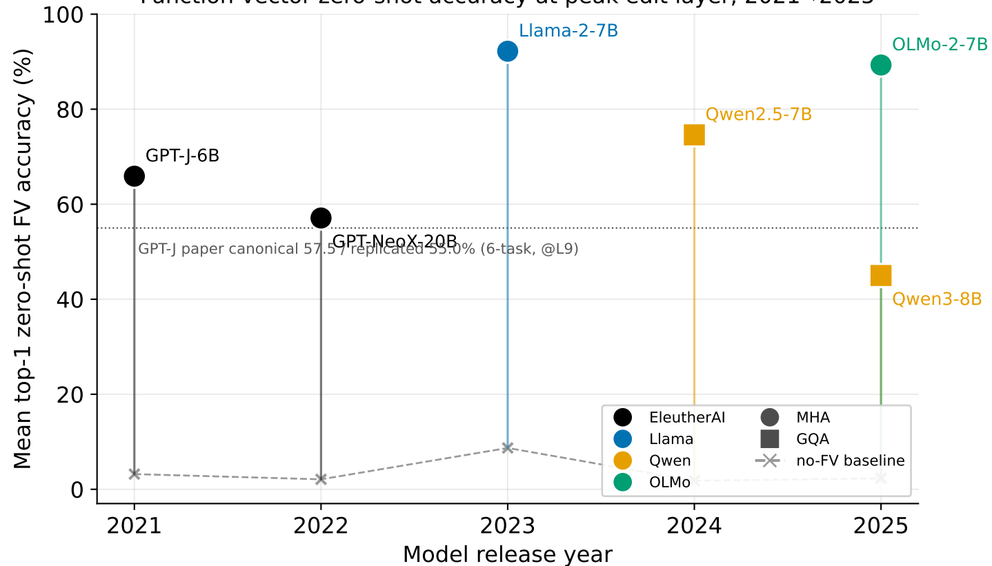
Function-vector zero-shot accuracy at peak edit layer, 2021→2025
