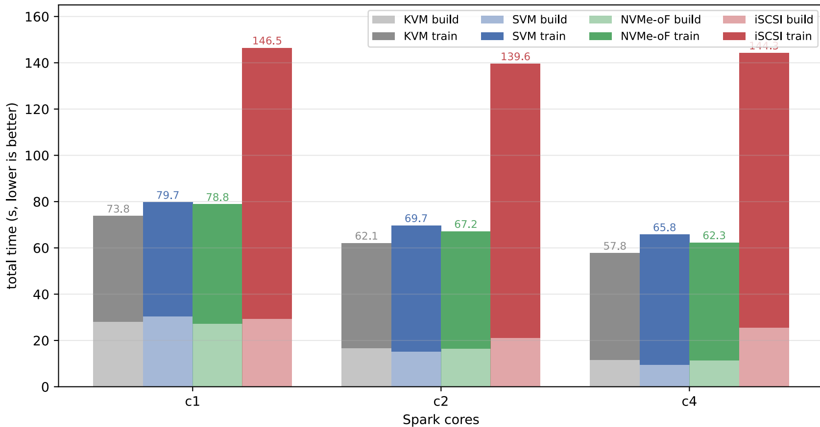
ALS-IO: total time stacked (build + train)
