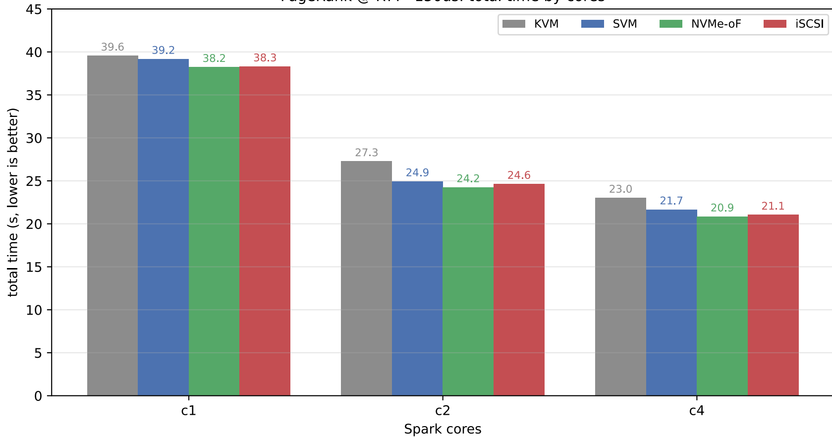
PageRank @ RTT~150us: total time by cores
