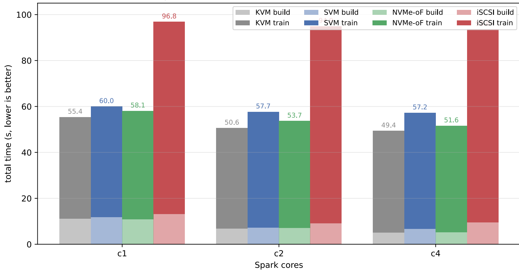
xgb (forced rescan): total time stacked (build + train)
