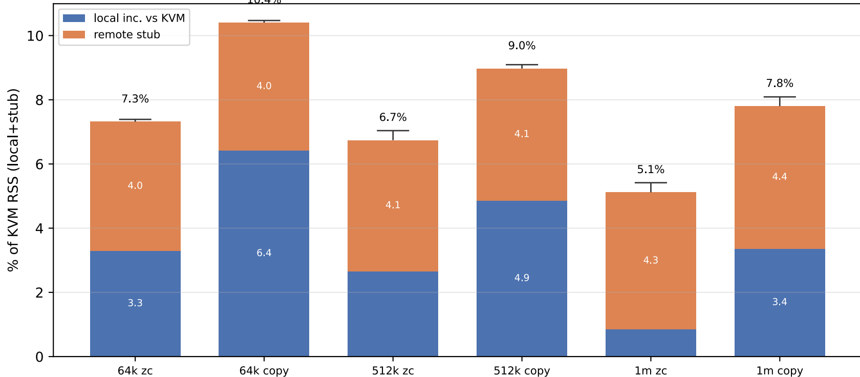
SVM virtio-remote RSS (local+stub) vs KVM: % increase fio randrw 7:3 d=1 l=256 P=off
