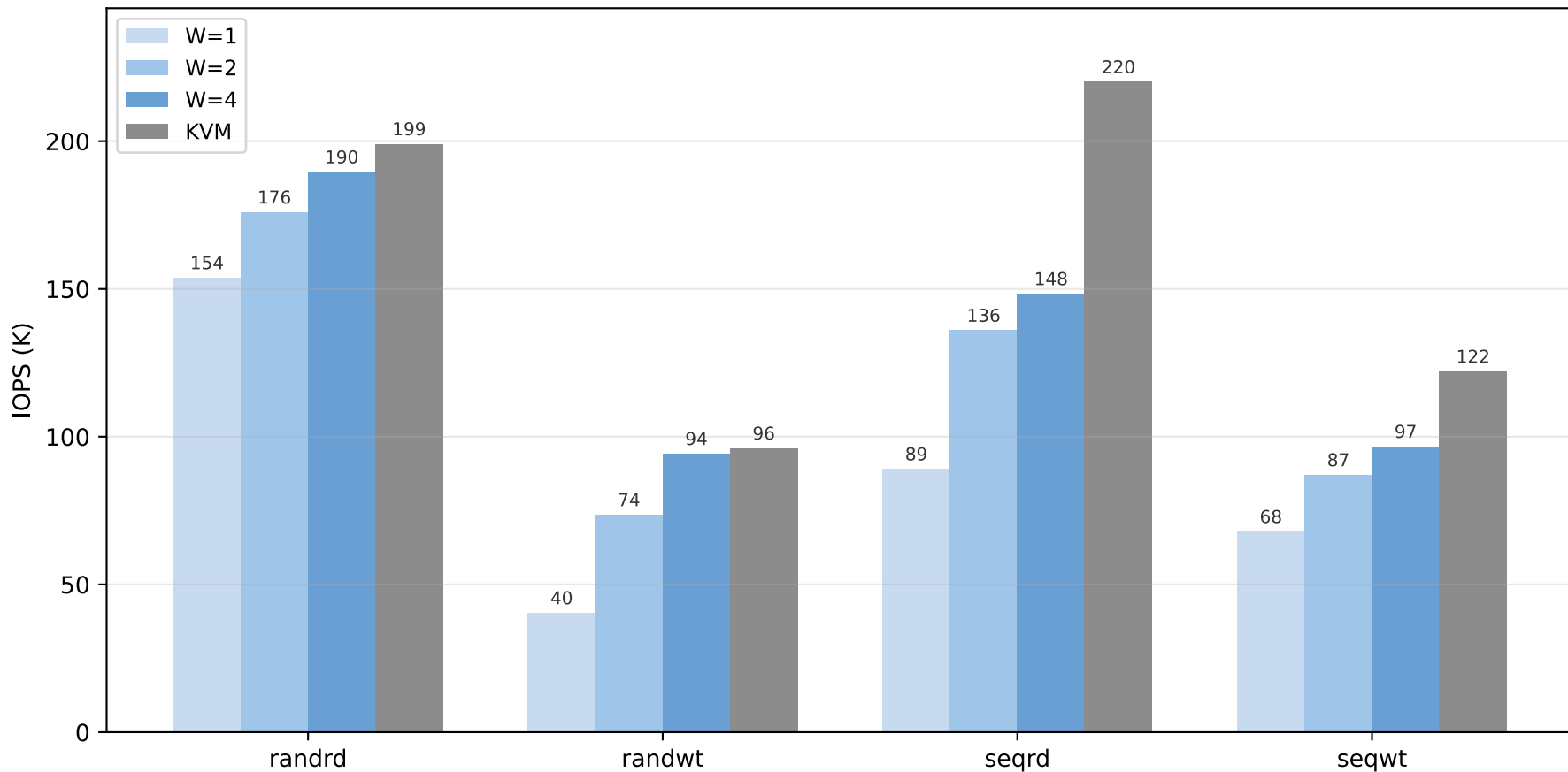
M2G: IOPS by workload (randread/randwrite/seqread/seqwrite, 4K) W=1/2/4 (t4/t5/t0) vs KVM
