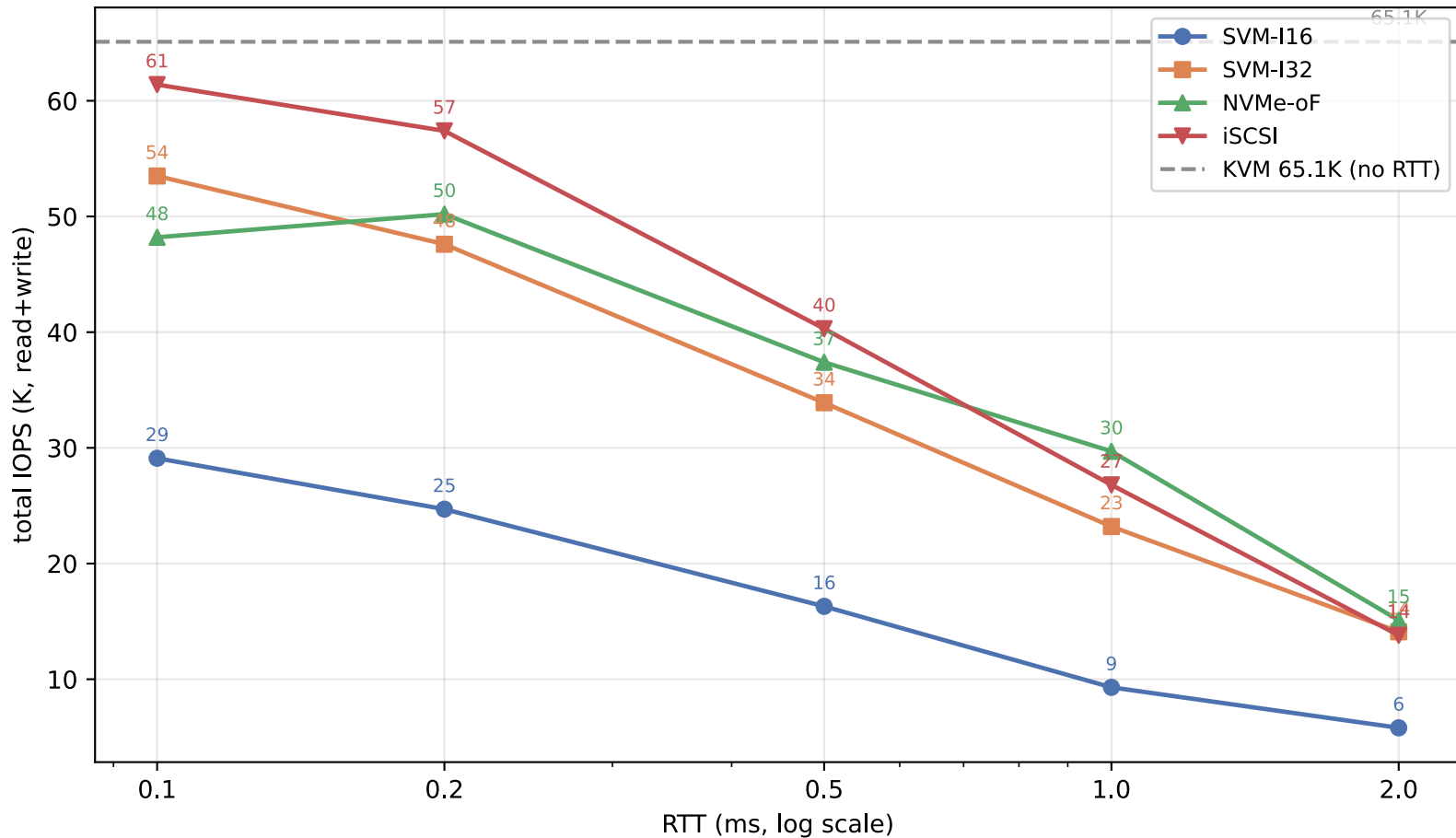
M3: IOPS vs RTT (randrw 70/30, 4K, iodepth=32, numjobs=1, 60s)
