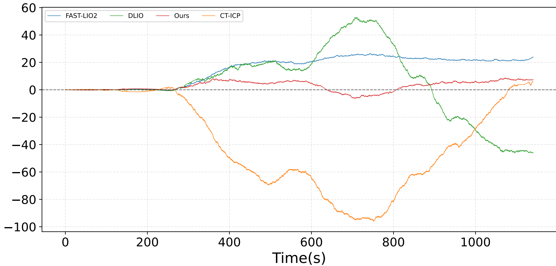
Y-direction error /m
