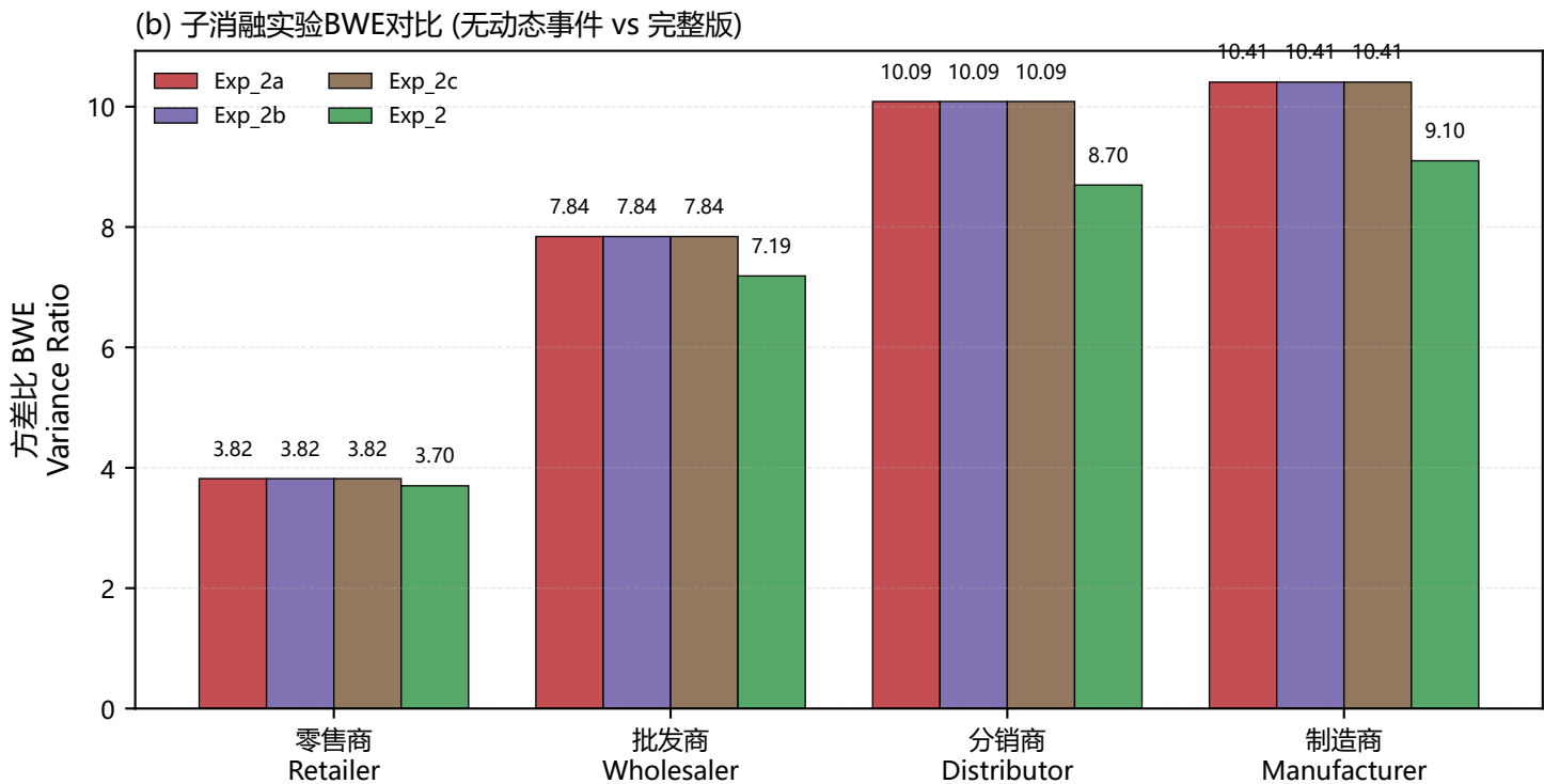
图2 消融实验剥离效应分解 Fig.2 Ablation effect decomposition (main + sub-ablation)
