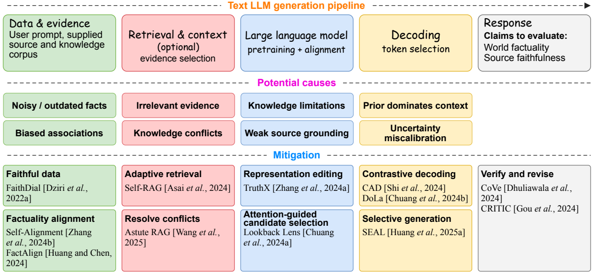
Figure 4: Potential causes and mitigation methods of hallucination in LLMs. Colors group stages of the generation pipeline; hybrid methods may span multiple stages.
