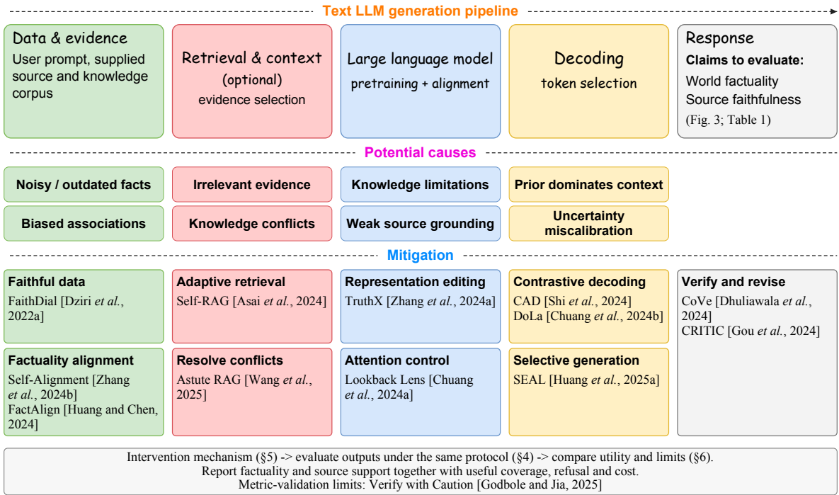
Figure 4: Potential failure sources and representative mitigation methods in text LLMs. Retrieval is optional. Stage associations summarize the literature; they do not establish one-to-one causal effects or guaranteed fixes. Evaluate outcomes using Fig. 3 and Table 1.
