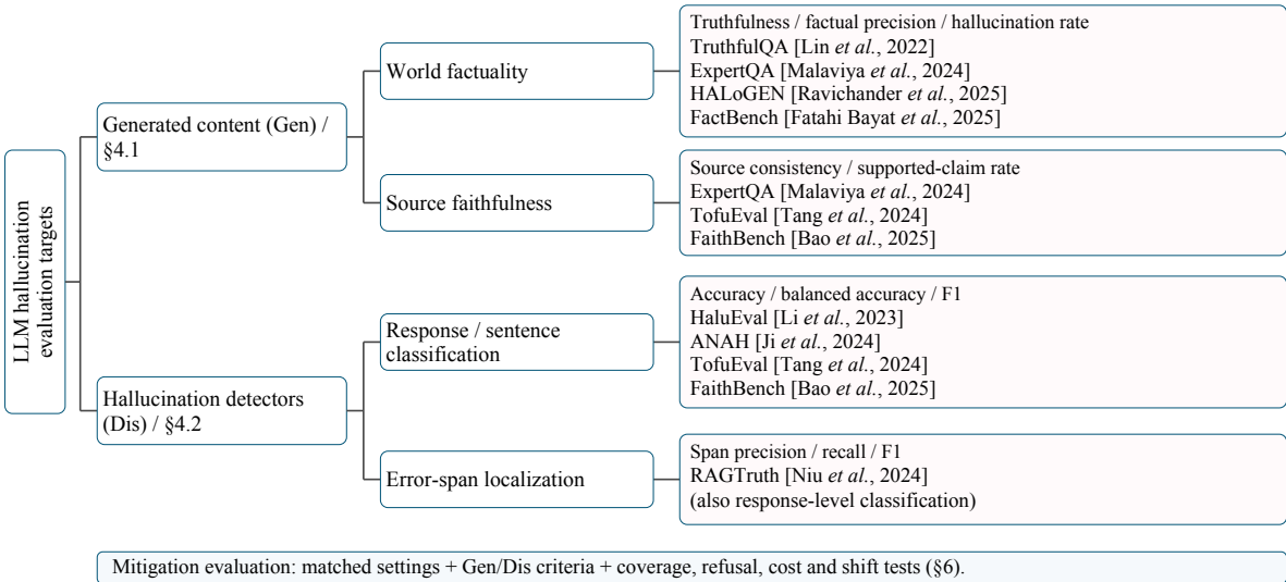
Figure 3: Taxonomy of evaluation targets and criteria with benchmark references. Gen evaluates generated content; Dis evaluates detectors against human labels. Criteria are not shared protocols; Table 1 gives benchmark-specific details. The same benchmark may support both targets.
