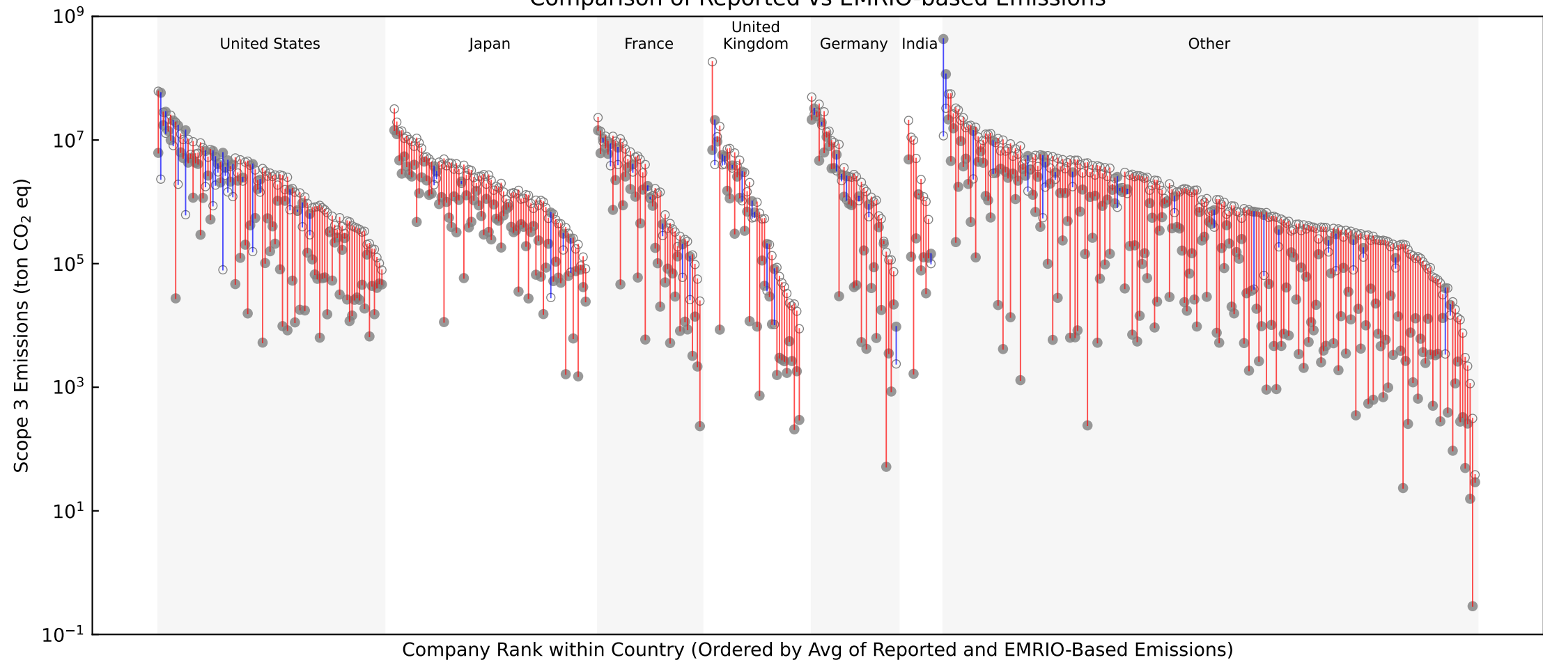
Comparison of Reported vs EMRIO-based Emissions
