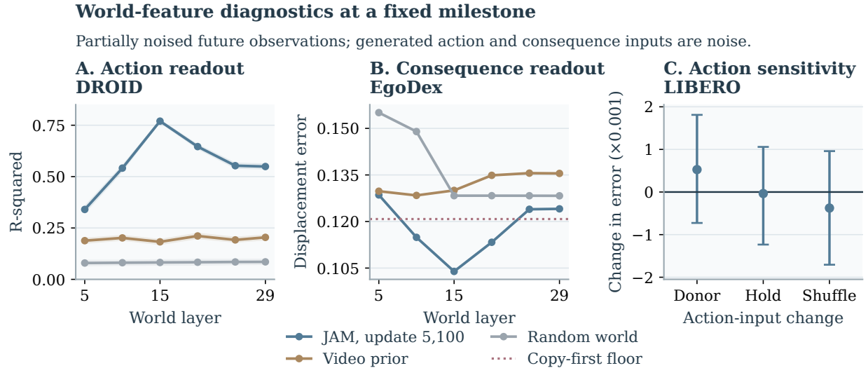
Figure 5: What is accessible in the world features? A–B: frozen-world ridge probes at every sampled depth, using partially noised future observations and fully corrupted action and consequence inputs. The held-out corpus windows are split into 2,800 probe-training and 1,200 probe-test windows; these probe splits can share episodes. Action-readout bands use 1,000 window-bootstrap resamples. C: consequence-error changes under substituted actions on 300 LIBERO windows, with paired 95% intervals. These intervals include zero. This panel measures input sensitivity; executed alternative-action futures are required for a causal prediction test.
