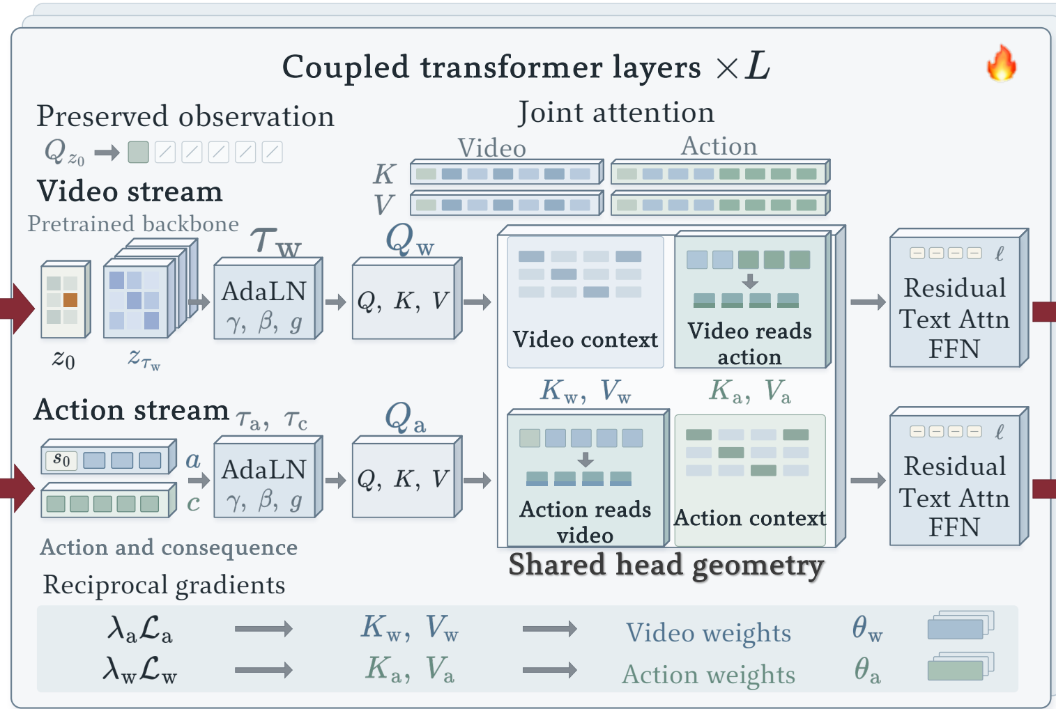
JAM: Joint Action-World Modeling
