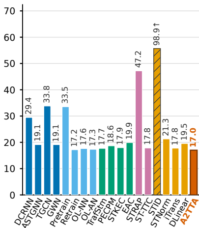
RMSE
