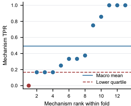
a Fold 0: 1 zero-detection mechanism(s)
