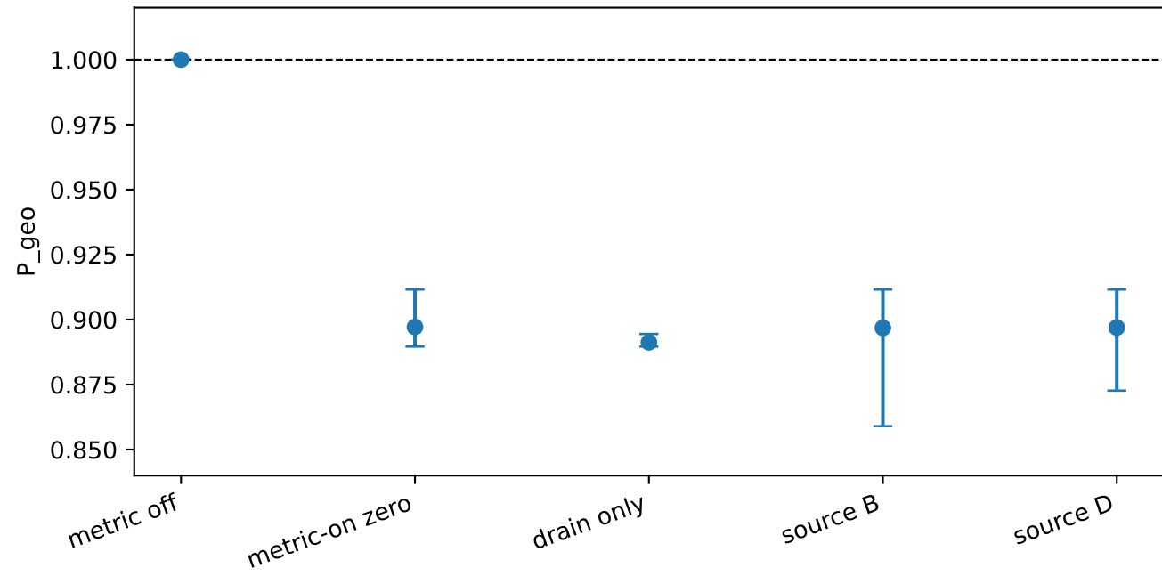
Newtonian-gauge CLASS benchmark and proxy branches
