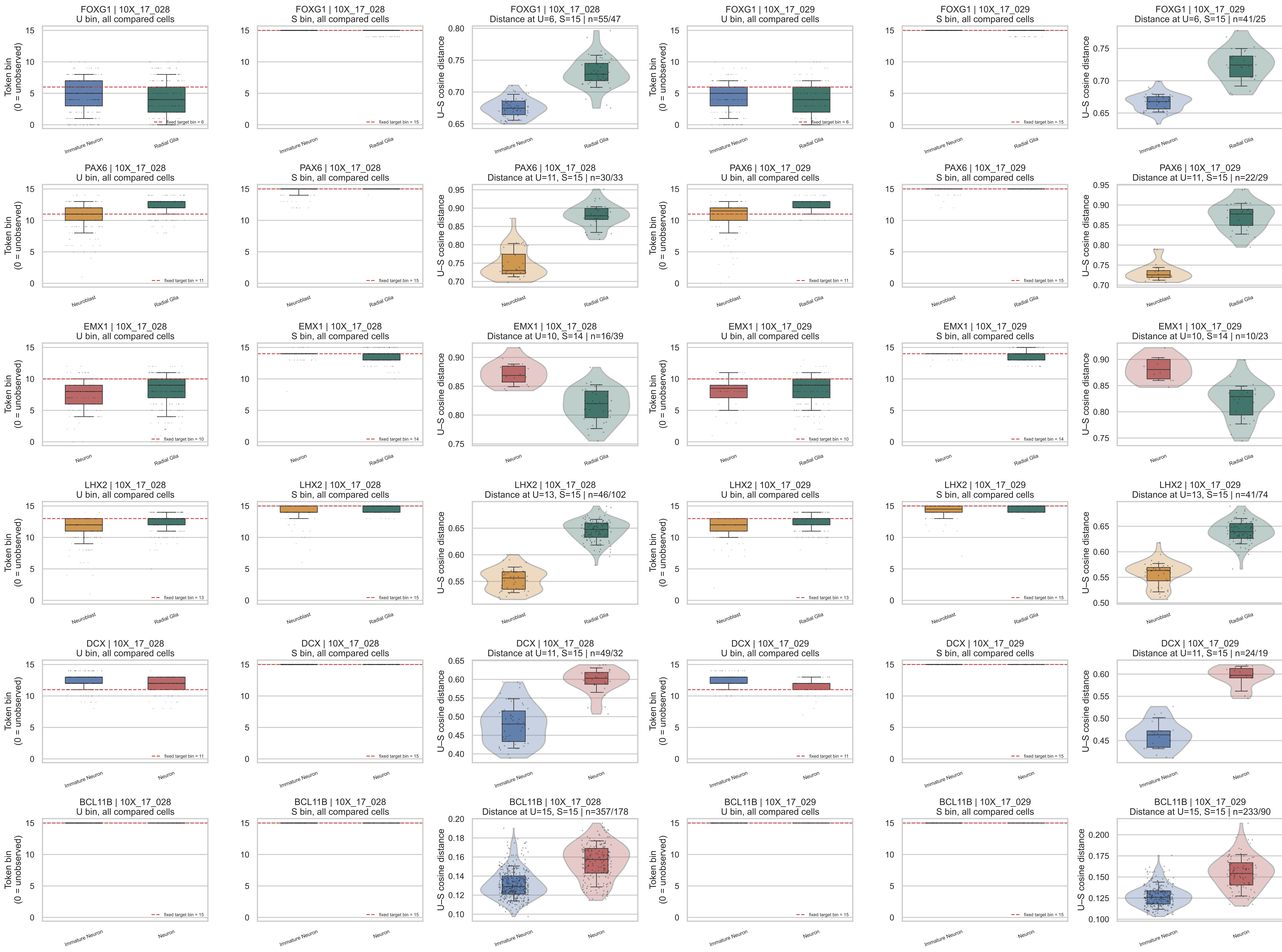
Same-sample input-bin context and fixed-token U–S distance Bin panels: all cells from the compared cell types; distance panels: exact U/S-bin subset only
