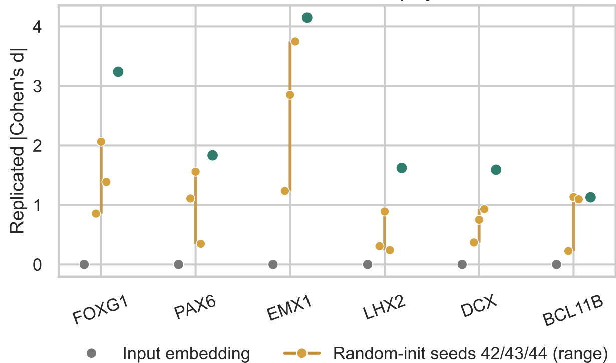
A Fixed all-ones hidden projection
