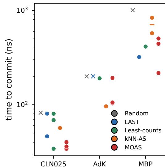
Time to committed visit
