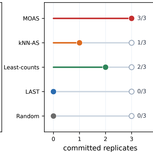
AdK committed success
