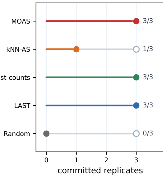
CLN025 committed success
