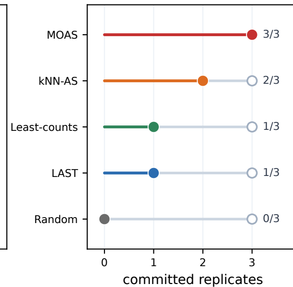
MBP committed success
