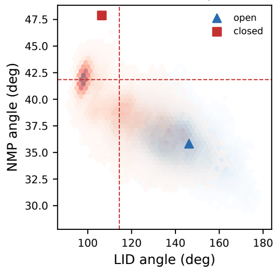
AdK CV density
