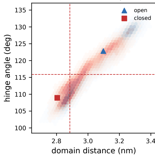
MBP CV density
