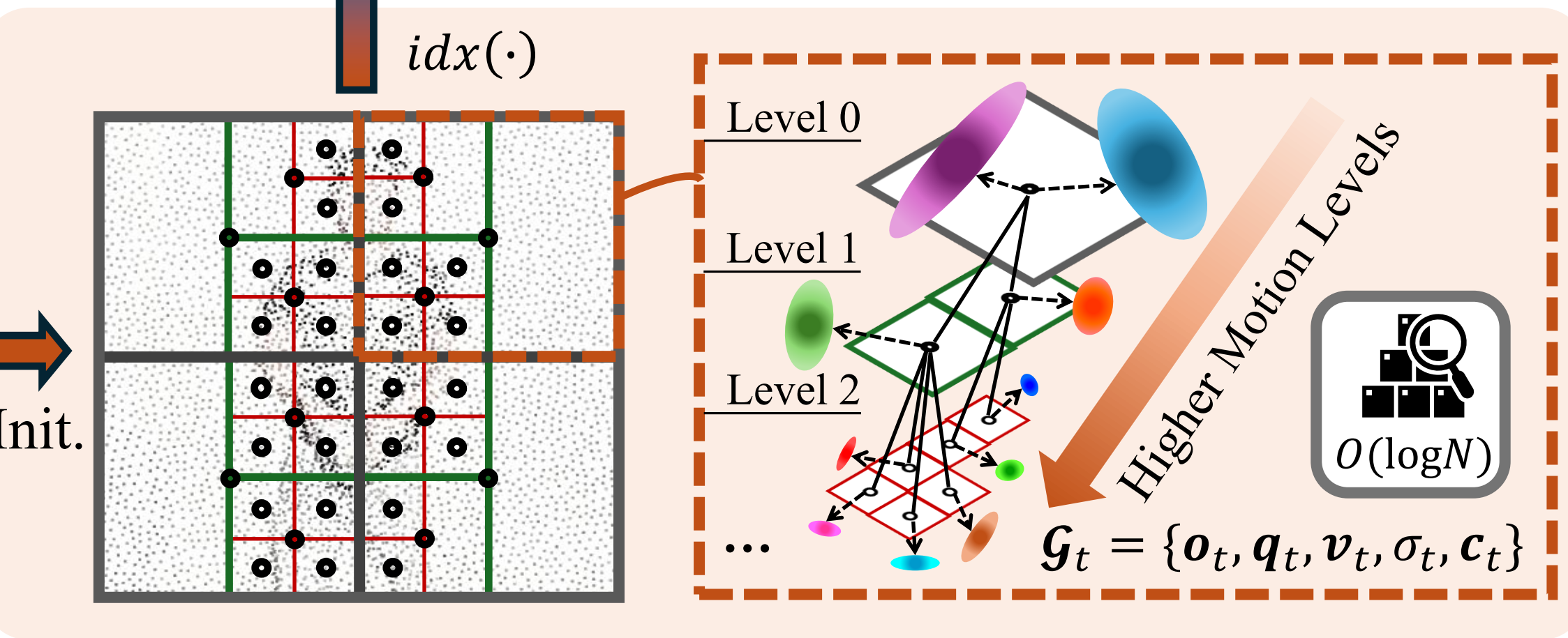
(a) Streaming Octree Representation
