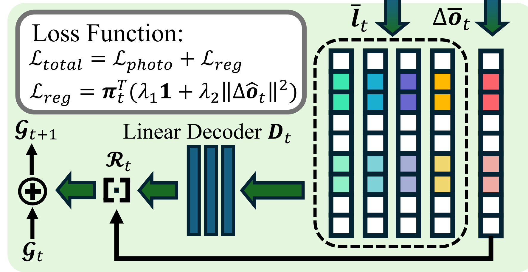
(c) Efficient End-to-end Training
