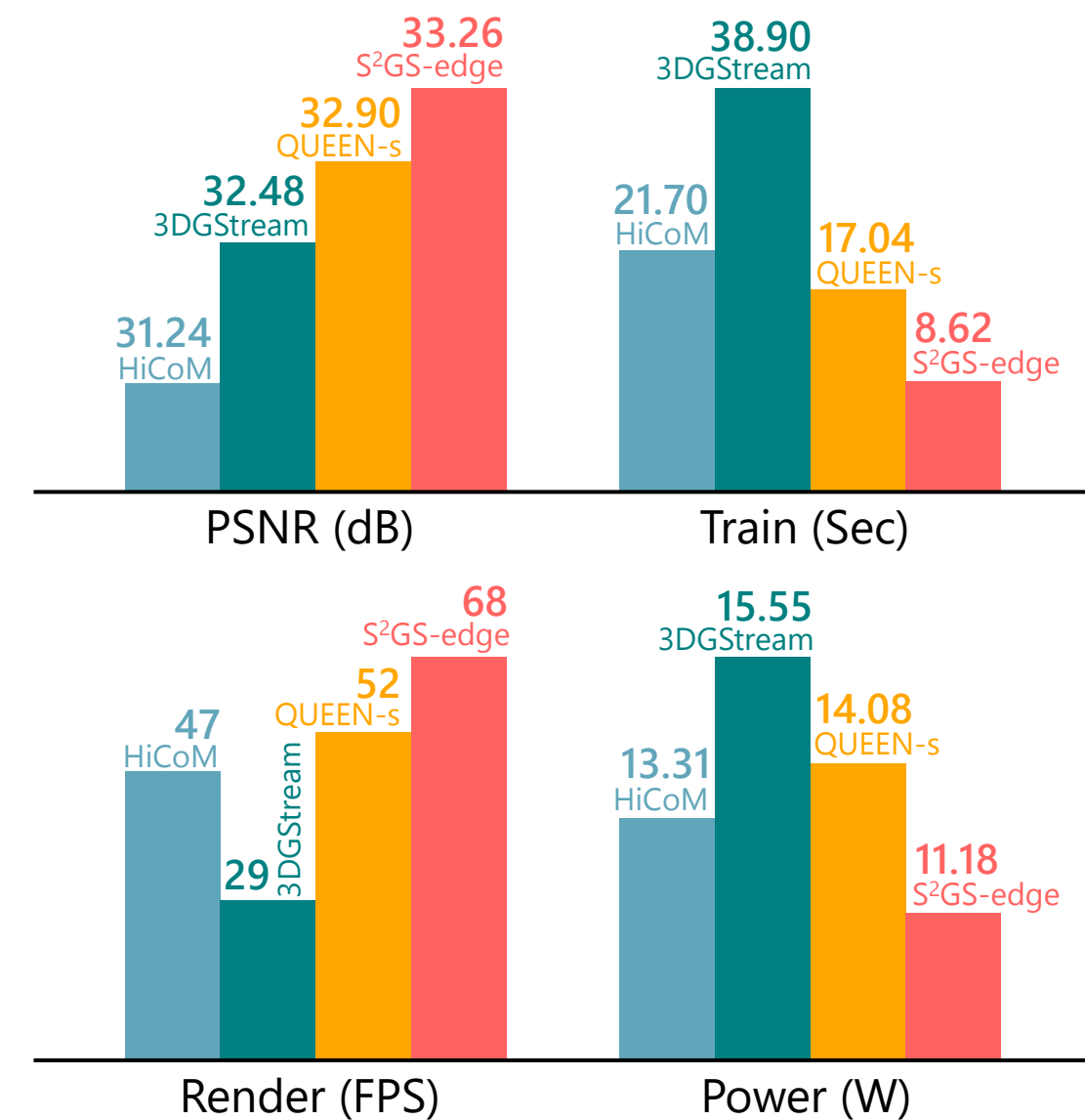
(c) Comparison on a NVIDIA AGX Orin
