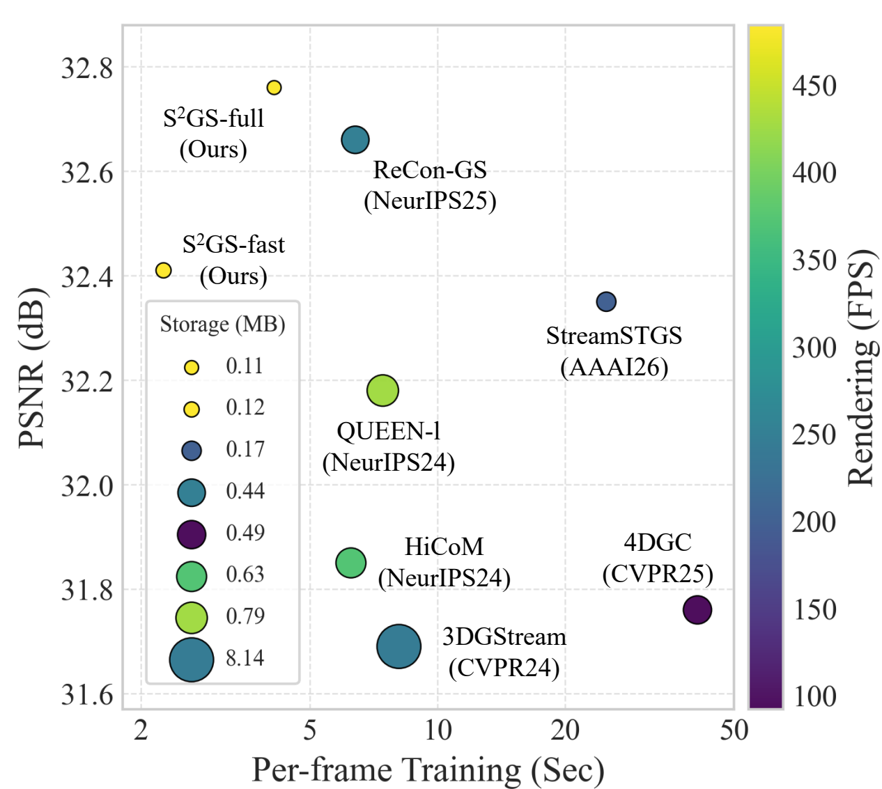
(a) Comparison on a NVIDIA RTX 4090 GPU
