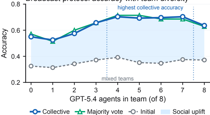
Broadcast protocol accuracy with team diversity
